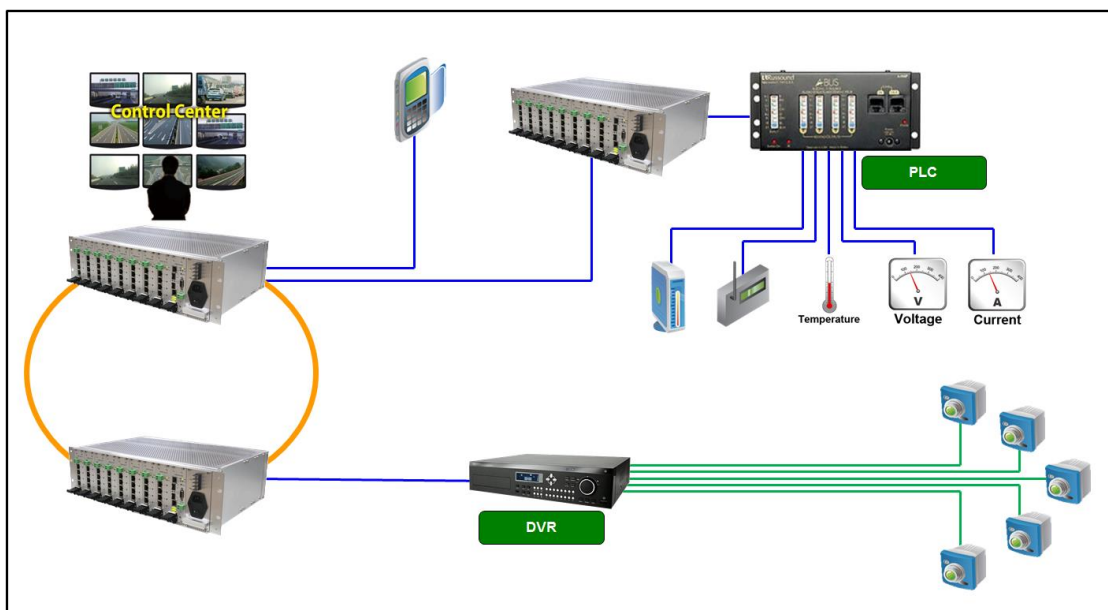
Network connection
