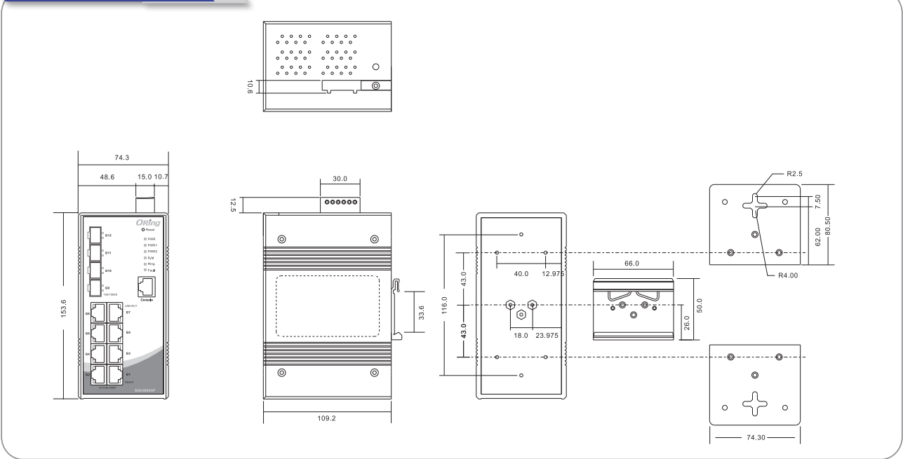
(Unit=mm)
