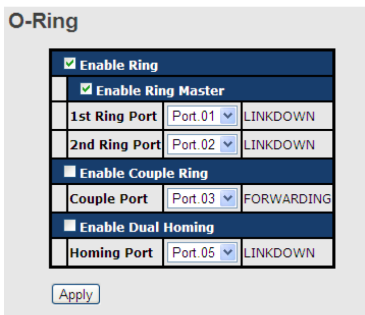
O-Ring interface
