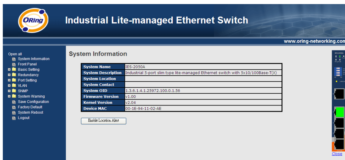
Main interface
